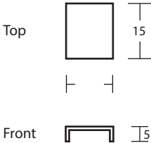
ARM TRAY W x 15D x 5H
