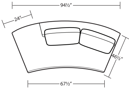
CURVED LSF BUMPER
