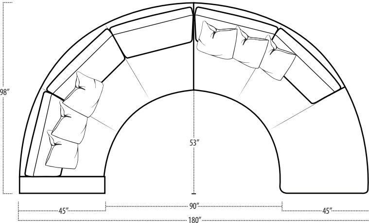
LAF 45 1 ARM CURVED SOFA + RSF 45 CURVED BUMPER
