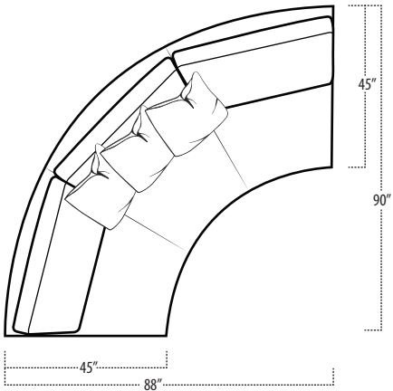
45 ARMLESS CURVED SOFA
