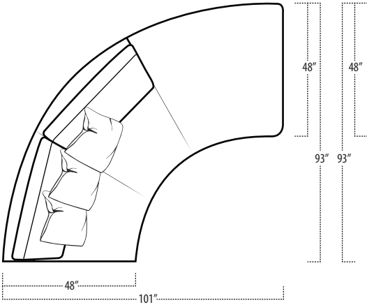
RSF 48 CURVED BUMPER
