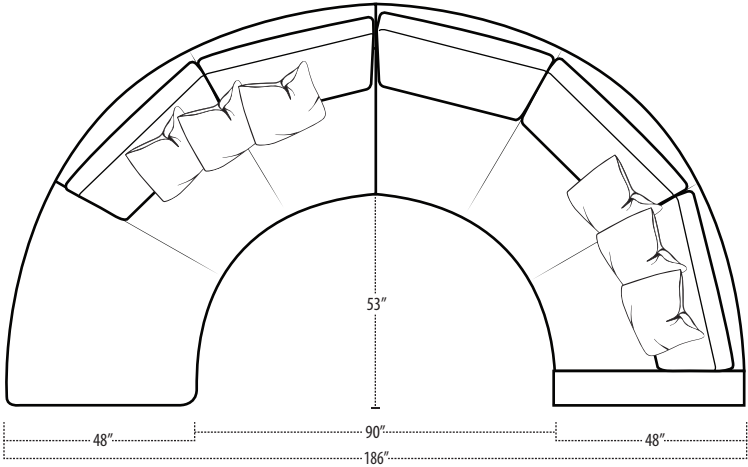
LSF 48 CURVED BUMPER + RAF 48 1 ARM CURVED SOFA
