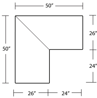
50 x 50 Angle Bench
