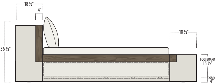
■ Top View Specifications | Scale: 1/4" = 1FT.
